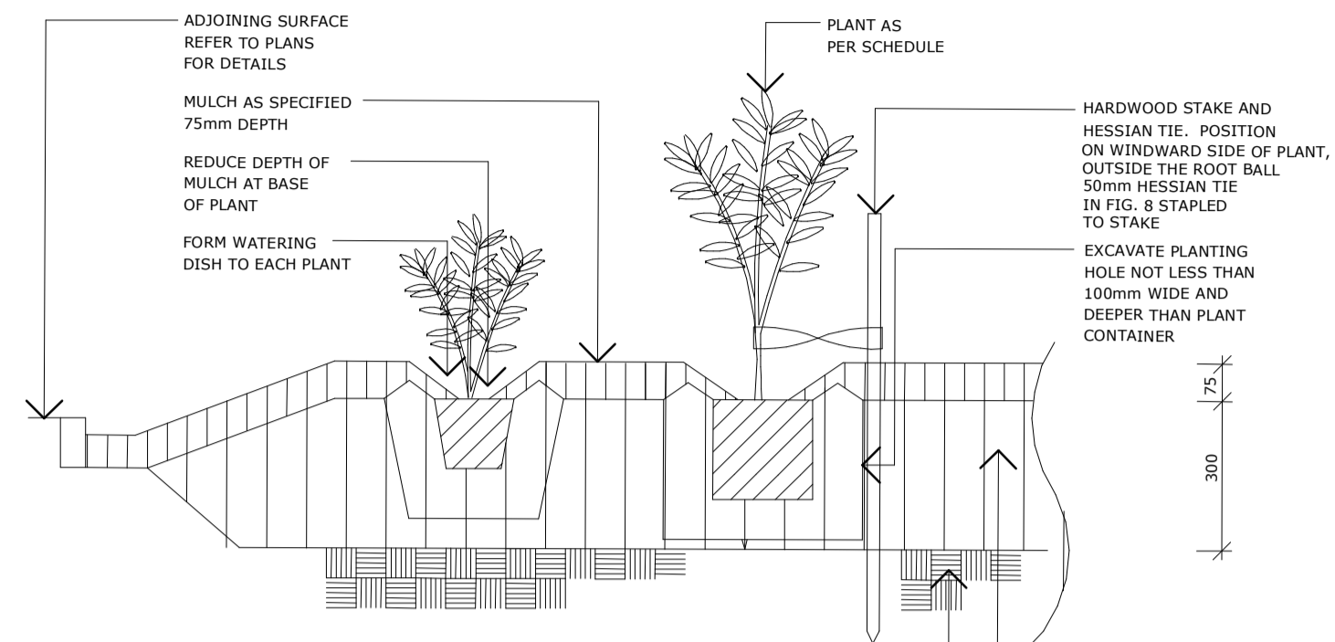
MASS PLANTING INTO NATURAL GROUND TYPICAL SECTION (NTS)
